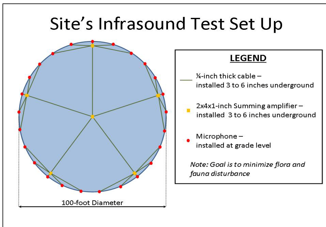
Figure 2. Infrasound test set up for borehole locations.
